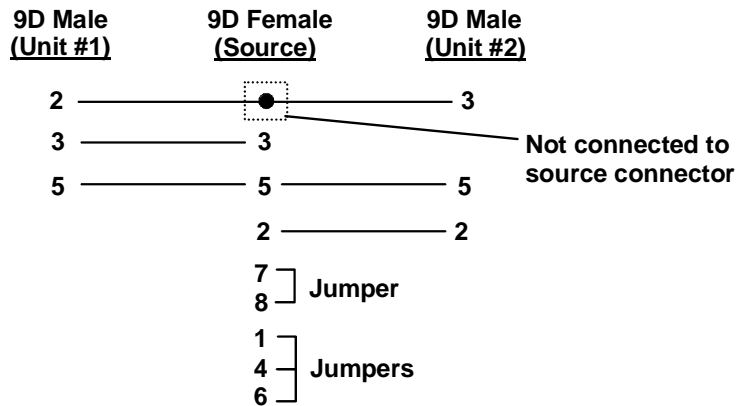
Figure 52- Pinout of Matrix-Y-1 cable
