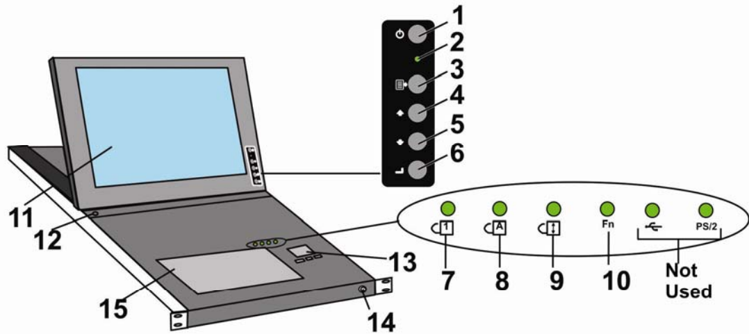
Front View RACKMUX-V17-N-8USBHD-IP
