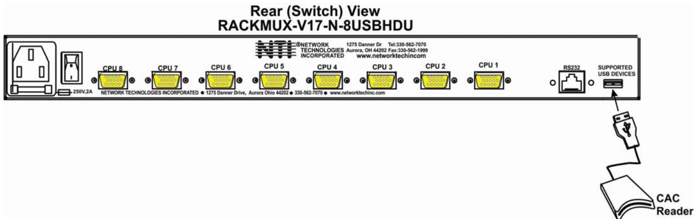
Figure 10- Install CAC card reader
