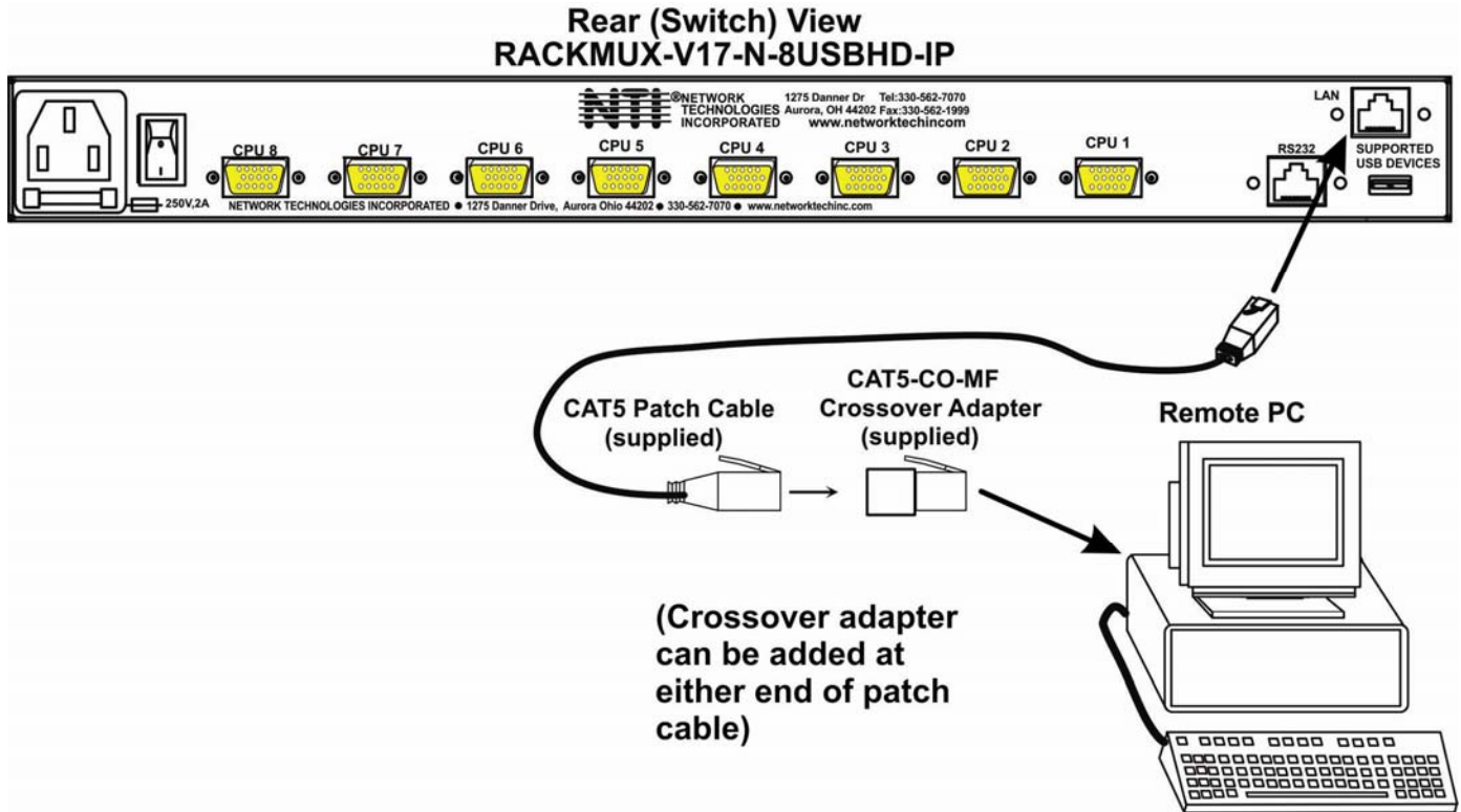
Figure 11- Connect Remote PC to KVM on IP at "LAN" port
