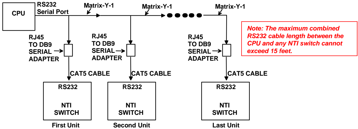
Figure 51- RS232 connection with Matrix-Y-1 cable
