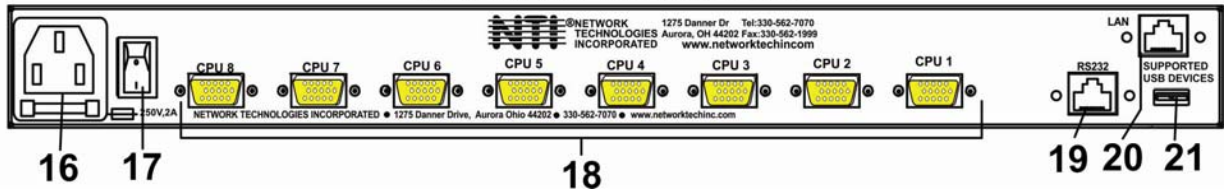
Rear (Switch) View RACKMUX-V17-N-8USBHD-IP
