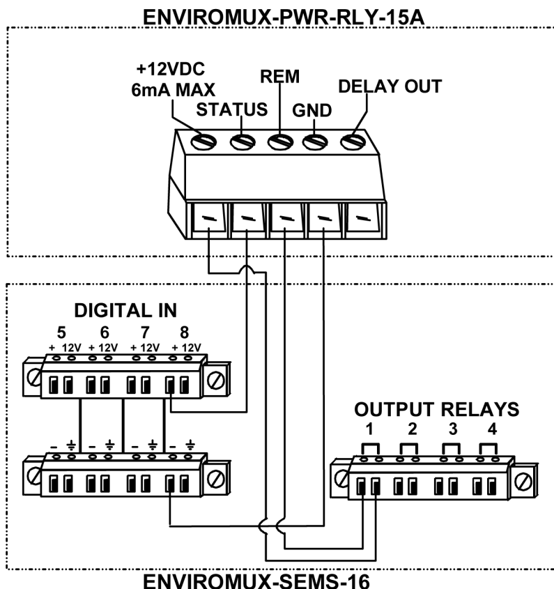
Figure 1- Wiring example
